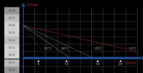
Fig : Self - Discharge Characteristics
